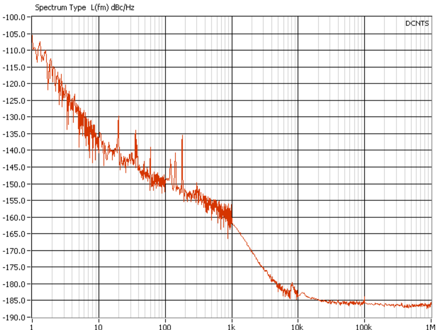
PN9000 Phase Noise Plot
